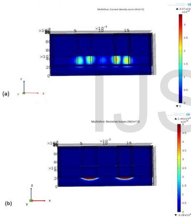
Fig. 5. a) Current density distribution. b) Losses distribution.
