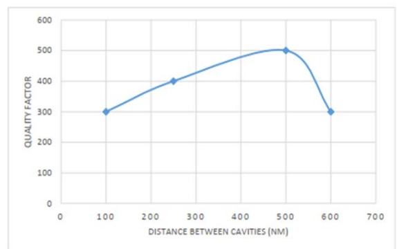
Fig. 7. Quality factor change with different distance between cavities.
