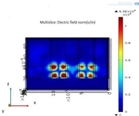
Fig. 4. Electric field distribution in the cavity.
