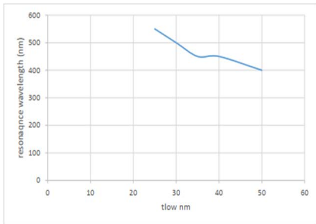
Fig. 8. Resonance wave length versus thickness of dielectric layer.
