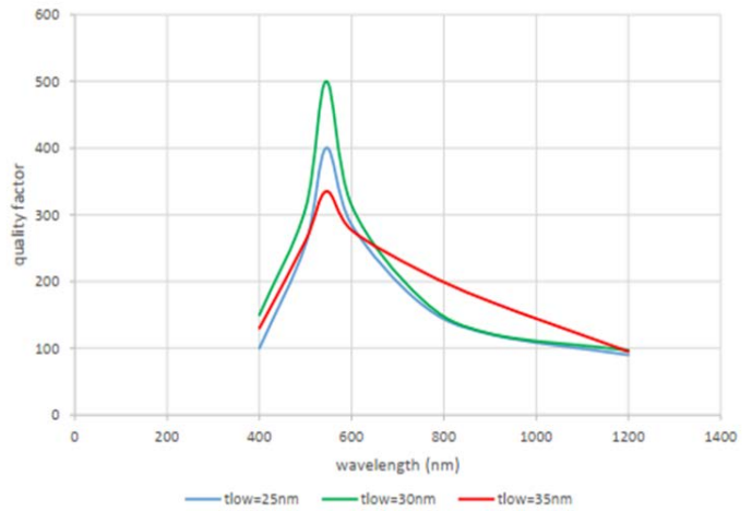
Fig. 9. Quality factor versus wavelength for different width of dielectric layer (using silver).
