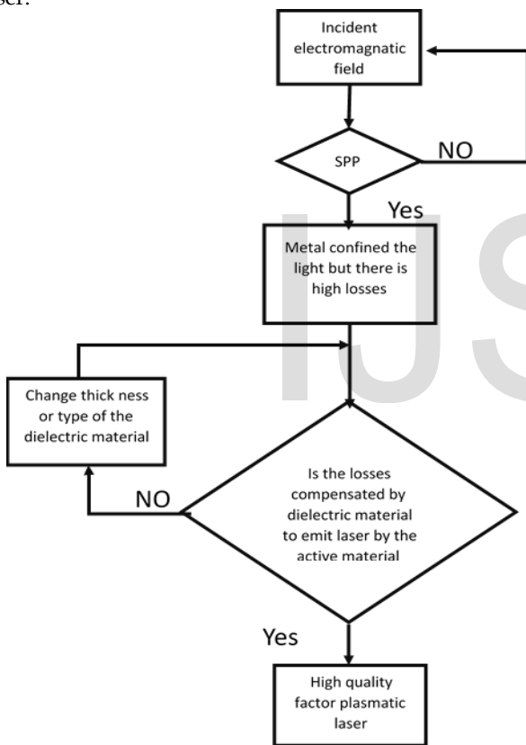
Fig. 2. Algorithm of plasmonic laser work.
