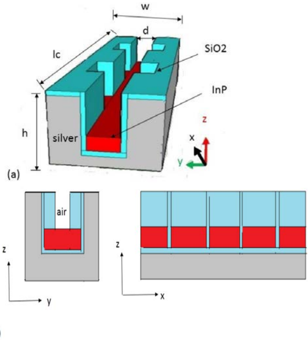
Fig. 3. a) Two cavity design b) Cross section of front and side of the cavity.
